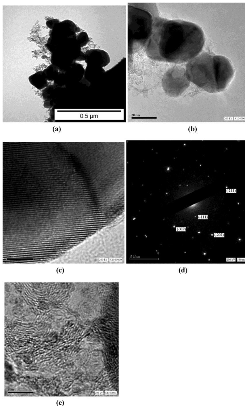
Figure 2. Transmission electron micrographs of (a) a MOPMF sample, (b) \text{MoO}_2 particles without carbon on the surface, (c) HR-TEM of a \text{MoO}_2 particle, (d) electron diffraction of same \text{MoO}_2 particle, and (e) carbon layers in a MOPMF sample.
